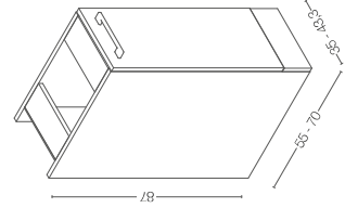
BASE ANTE A TERRA FLOOR-RESTING BASE DOOR
