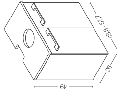
BASE LAVABO CON TOP WASHBASIN BASE WITH TOP
