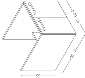
BASE PORTALAVABO 2 ANTE SOSPESA SUSPENDED WASHBASIN CABINET BASE 2 DOORS
