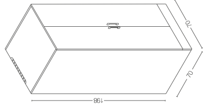
COLONNA LAVATRICE WASHING MACHINE COLUMN
