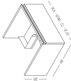
BASE LAVABO WASHBASIN BASE
