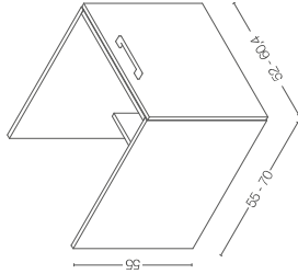
BASE PORTALAVABO CASSETTONE WASHBASIN CABINET BASE CHEST OF DRAWERS
