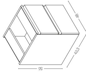
BASE CASSETTI BASE DRAWERS
